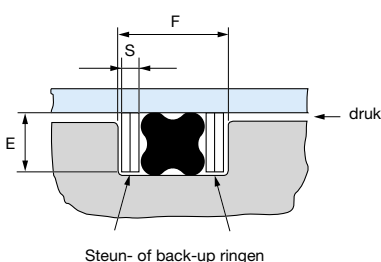
Steun- of back-up ringen
